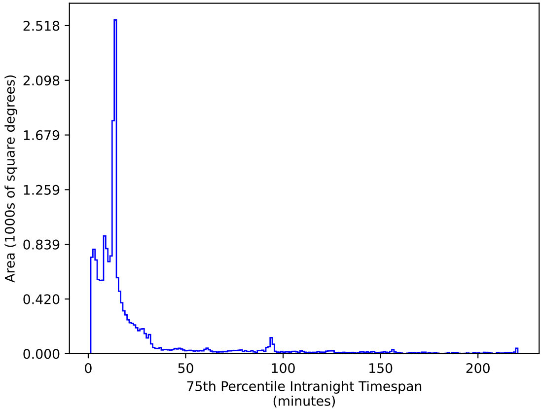
ddf_acor_sf10_lsf40_lsr10_v3.4_10yrs WFD i band: 75th Percentile Intranight Timespan
