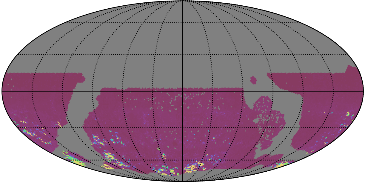
ddf_acor_sf10_lsf40_lsr10_v3.4_10yrs WFD gr bands: 75th Percentile Intranight Timespan
