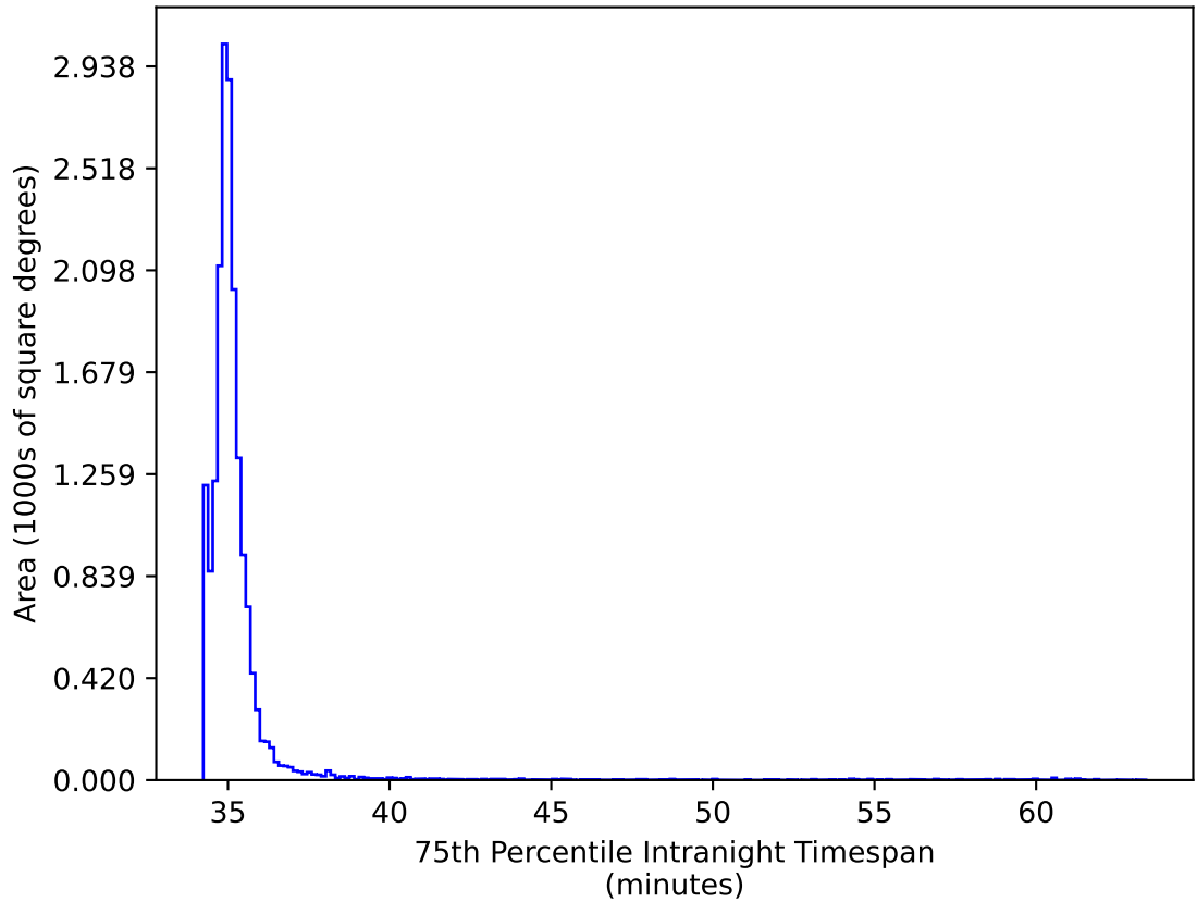
ddf_acor_sf10_lsf40_lsr10_v3.4_10yrs WFD gr bands: 75th Percentile Intranight Timespan
