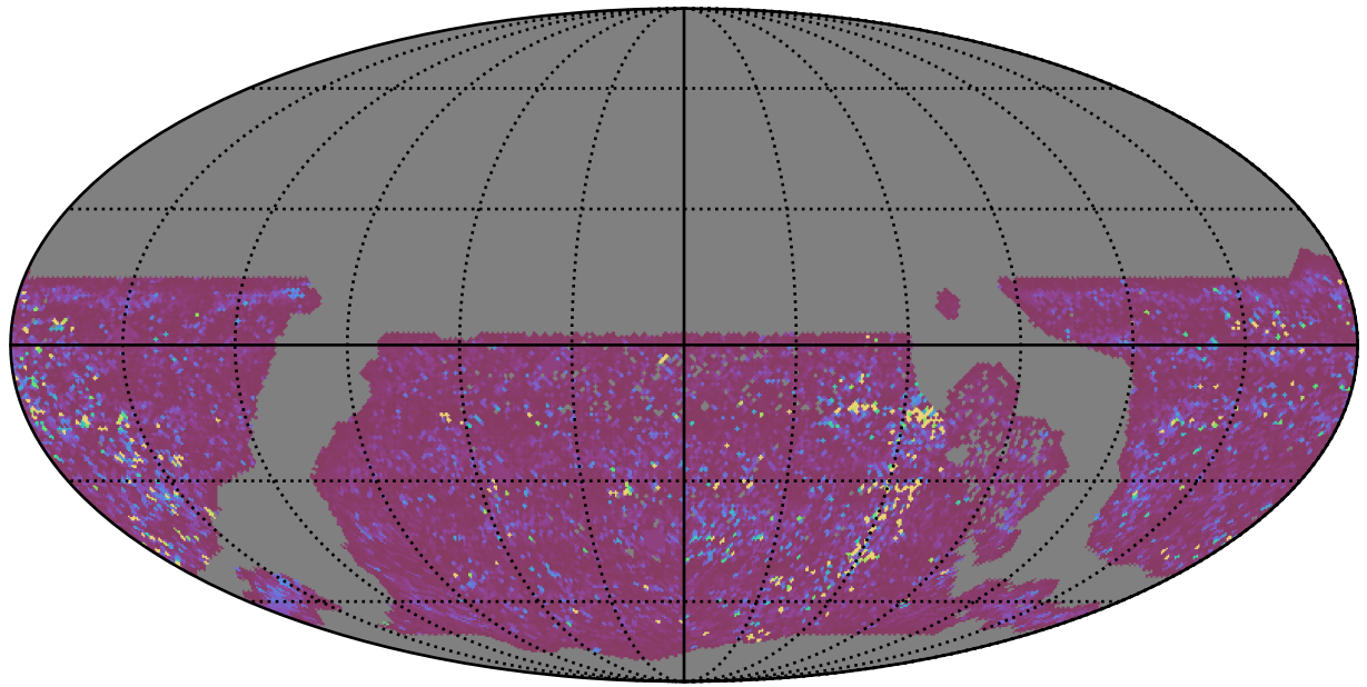
ddf_acor_sf10_lsf40_lsr10_v3.4_10yrs WFD g band: 75th Percentile Intranight Timespan
