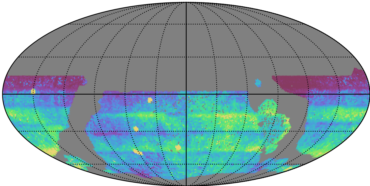
ddf_acor_sf10_lsf40_lsr10_v3.4_10yrs WFD all bands: 75th Percentile Intranight Timespan
