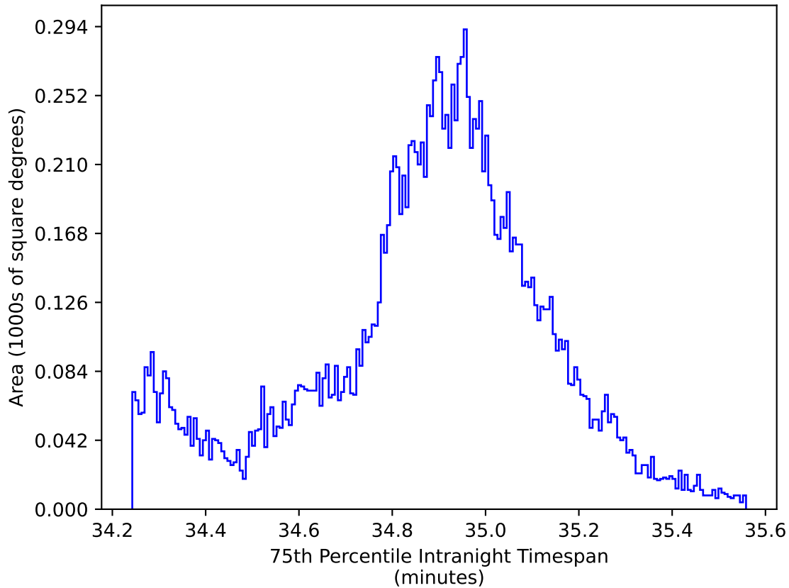
ddf_acor_sf10_lsf40_lsr10_v3.4_10yrs WFD all bands: 75th Percentile Intranight Timespan
