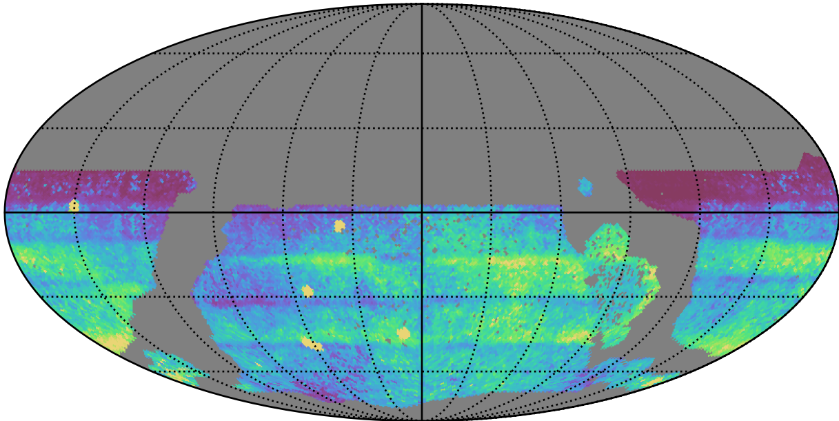
ddf_acor_sf10_lsf40_lsr10_v3.4_10yrs WFD: 75th Percentile Intranight Timespan
