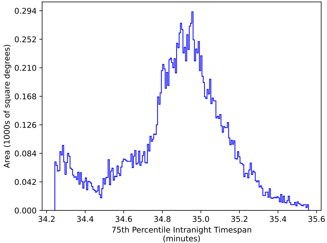
ddf_acor_sf10_lsf40_lsr10_v3.4_10yrs WFD: 75th Percentile Intranight Timespan
