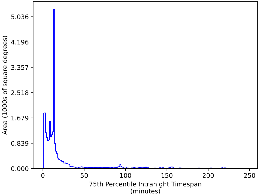
ddf_acor_sf10_lsf40_lsr10_v3.4_10yrs All sky z band: 75th Percentile Intranight Timespan
