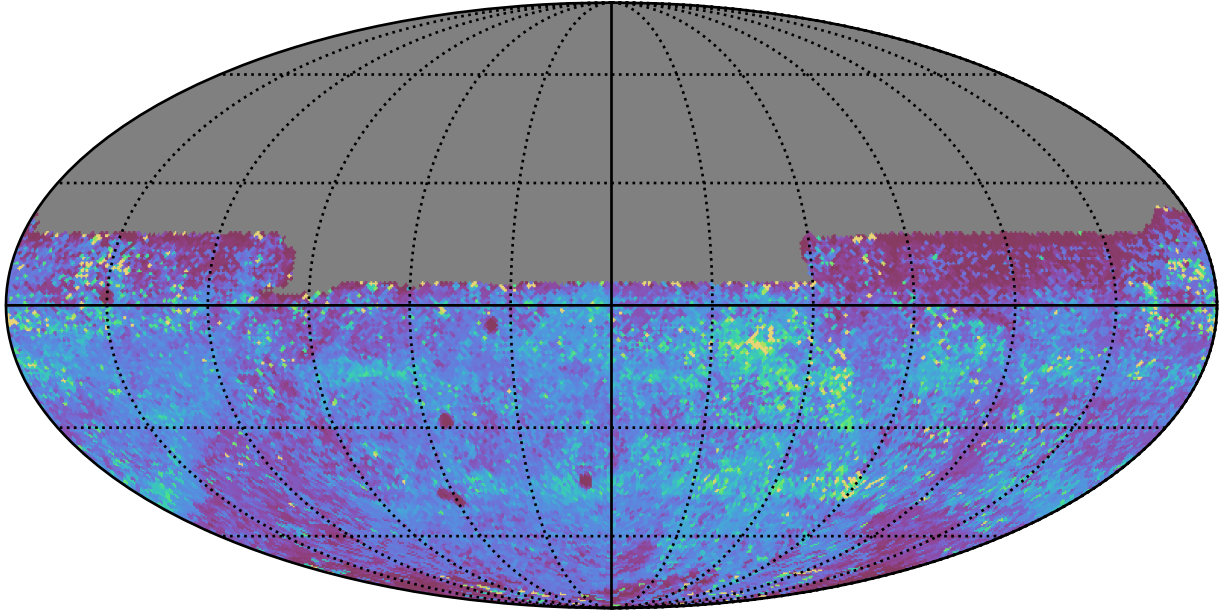
ddf_acor_sf10_lsf40_lsr10_v3.4_10yrs All sky y band: 75th Percentile Intranight Timespan
