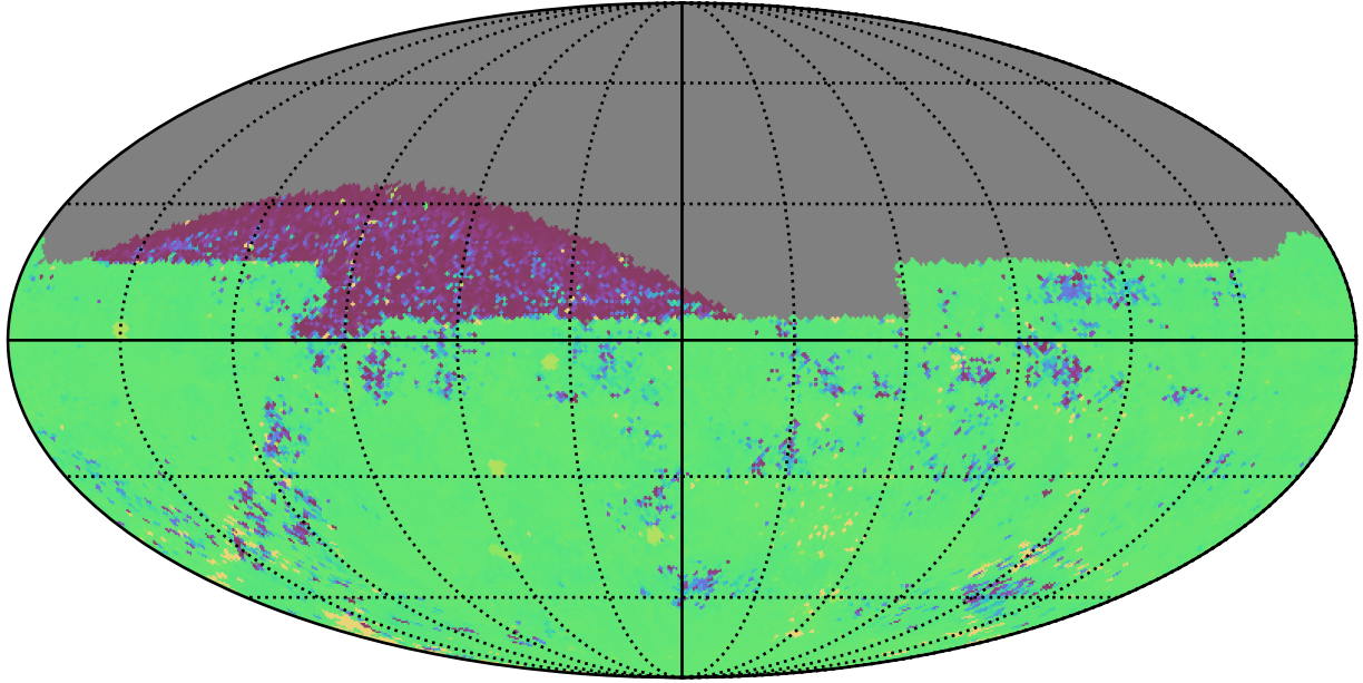
ddf_acor_sf10_lsf40_lsr10_v3.4_10yrs All sky ug bands: 75th Percentile Intranight Timespan
