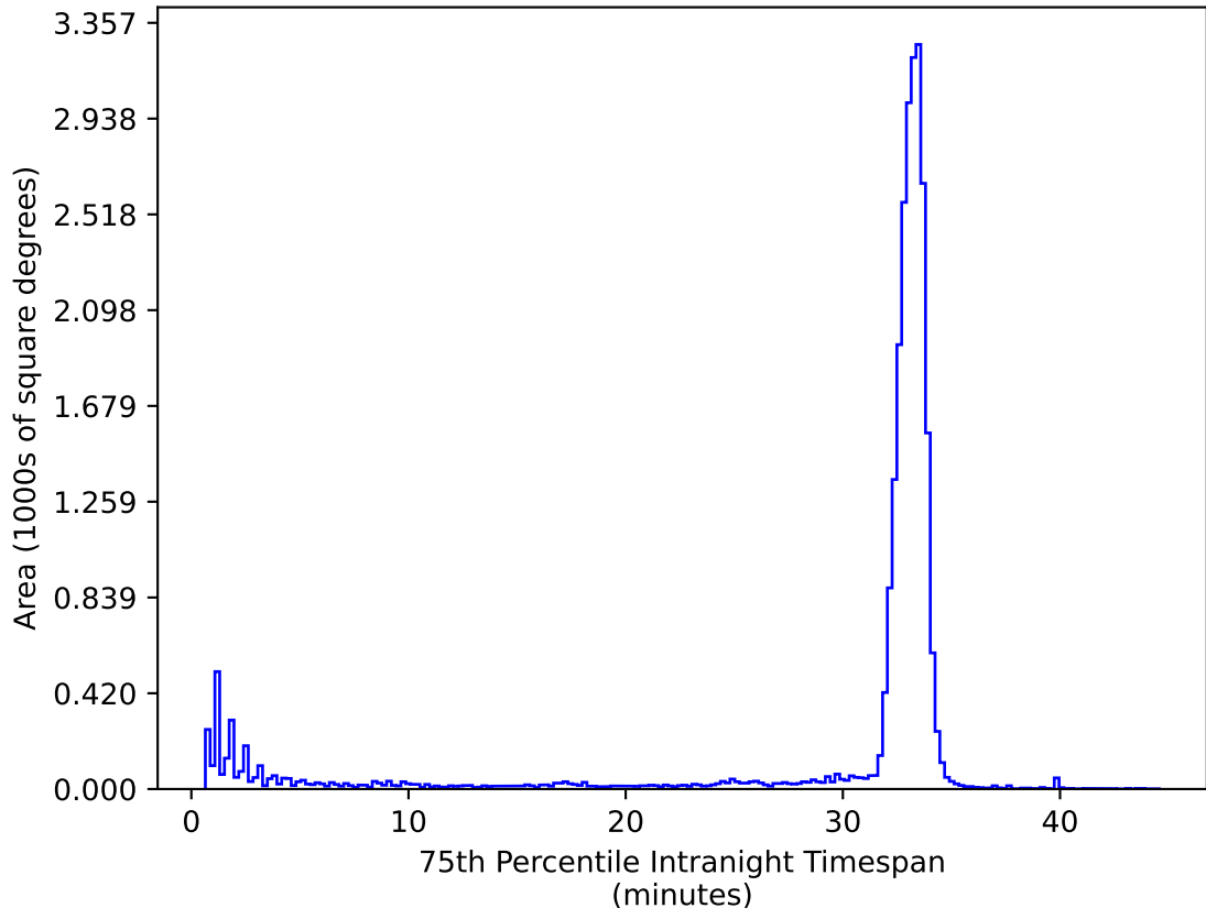
ddf_acor_sf10_lsf40_lsr10_v3.4_10yrs All sky ug bands: 75th Percentile Intranight Timespan
