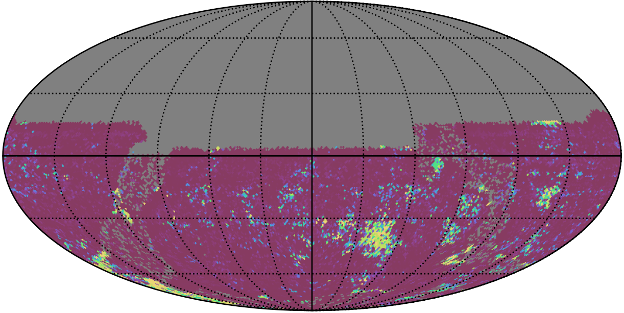
ddf_acor_sf10_lsf40_lsr10_v3.4_10yrs All sky u band: 75th Percentile Intranight Timespan
