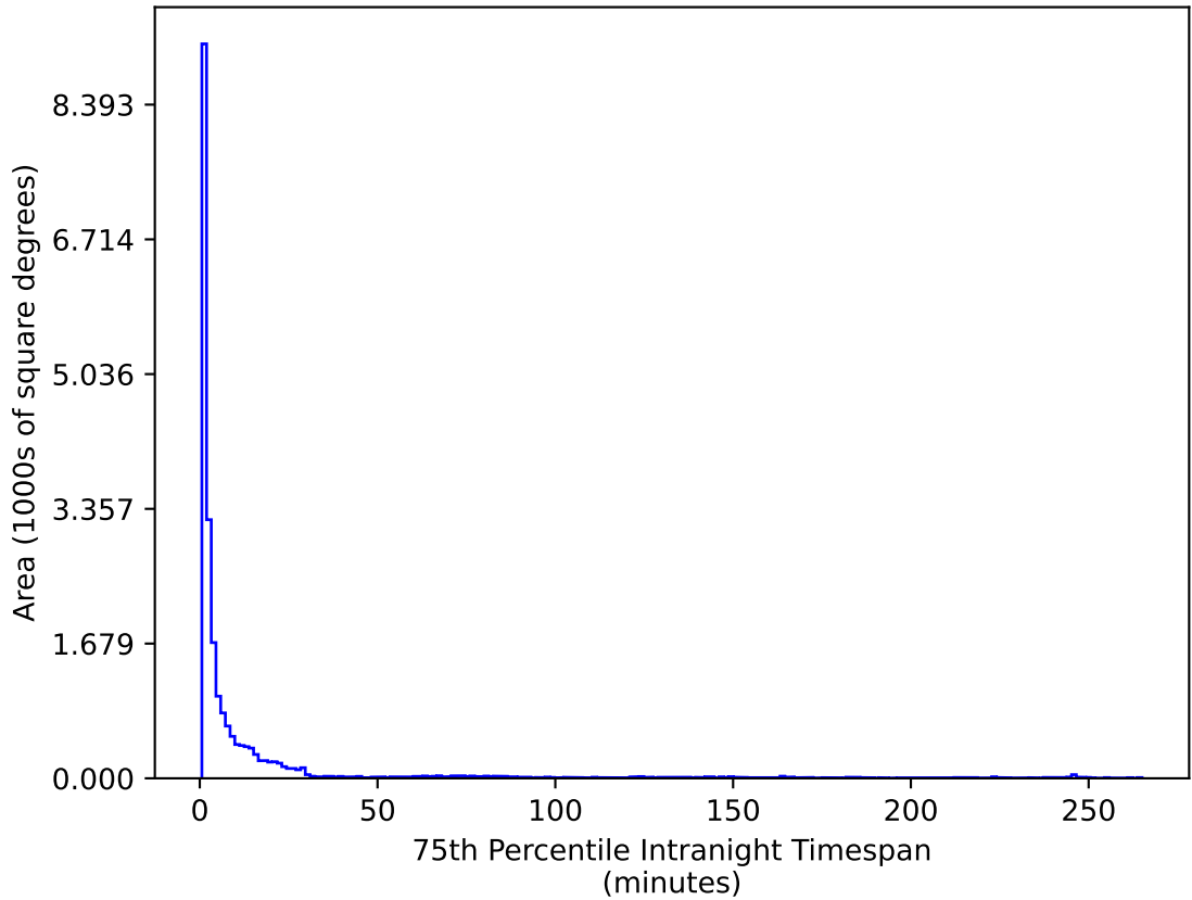
ddf_acor_sf10_lsf40_lsr10_v3.4_10yrs All sky u band: 75th Percentile Intranight Timespan
