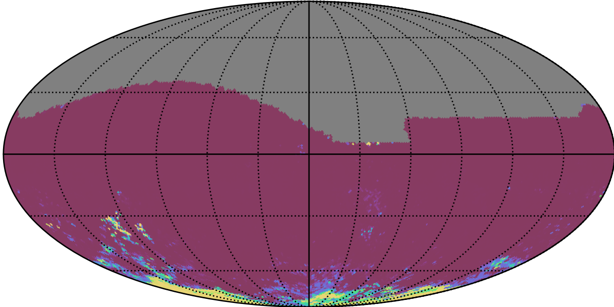
ddf_acor_sf10_lsf40_lsr10_v3.4_10yrs All sky ri bands: 75th Percentile Intranight Timespan
