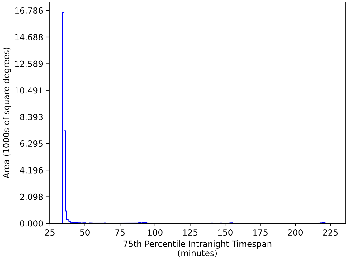
ddf_acor_sf10_lsf40_lsr10_v3.4_10yrs All sky ri bands: 75th Percentile Intranight Timespan
