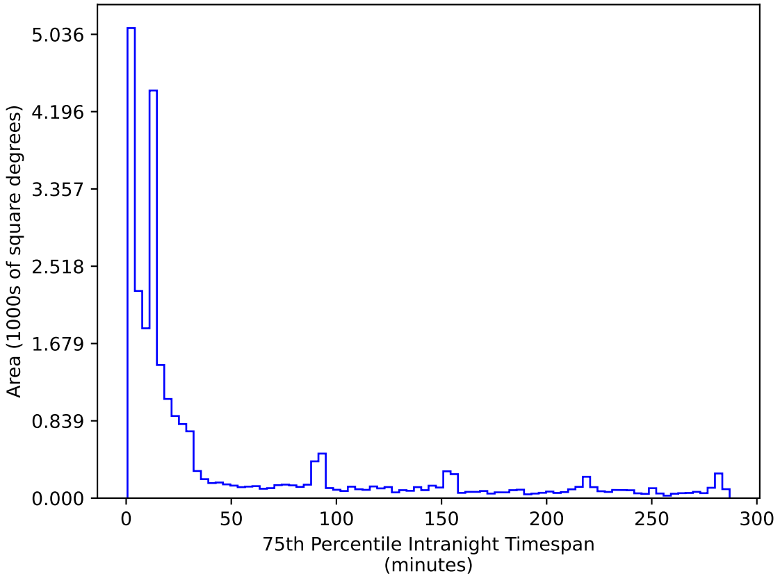
ddf_acor_sf10_lsf40_lsr10_v3.4_10yrs All sky r band: 75th Percentile Intranight Timespan
