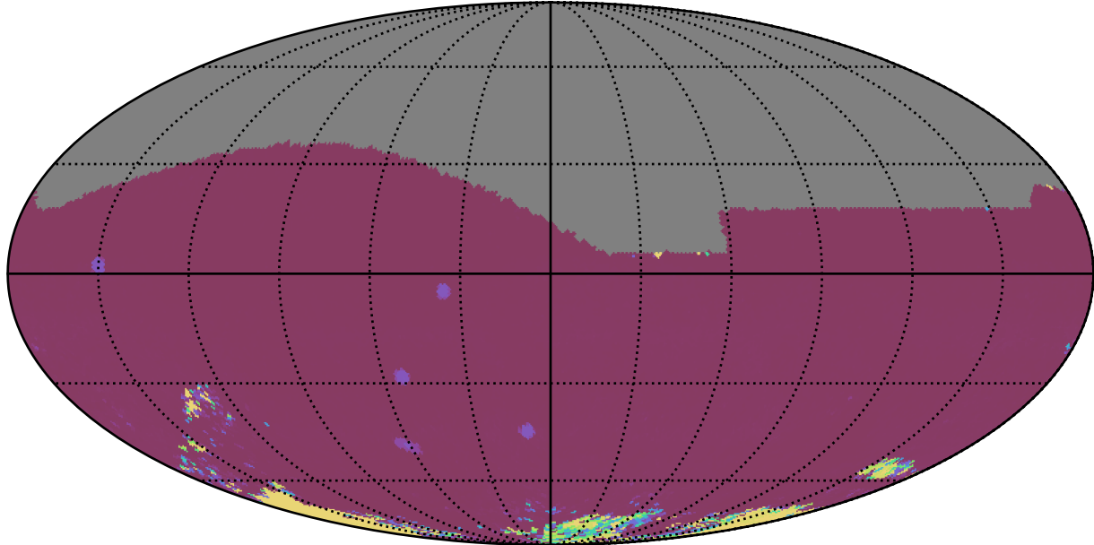
ddf_acor_sf10_lsf40_lsr10_v3.4_10yrs All sky iz bands: 75th Percentile Intranight Timespan
