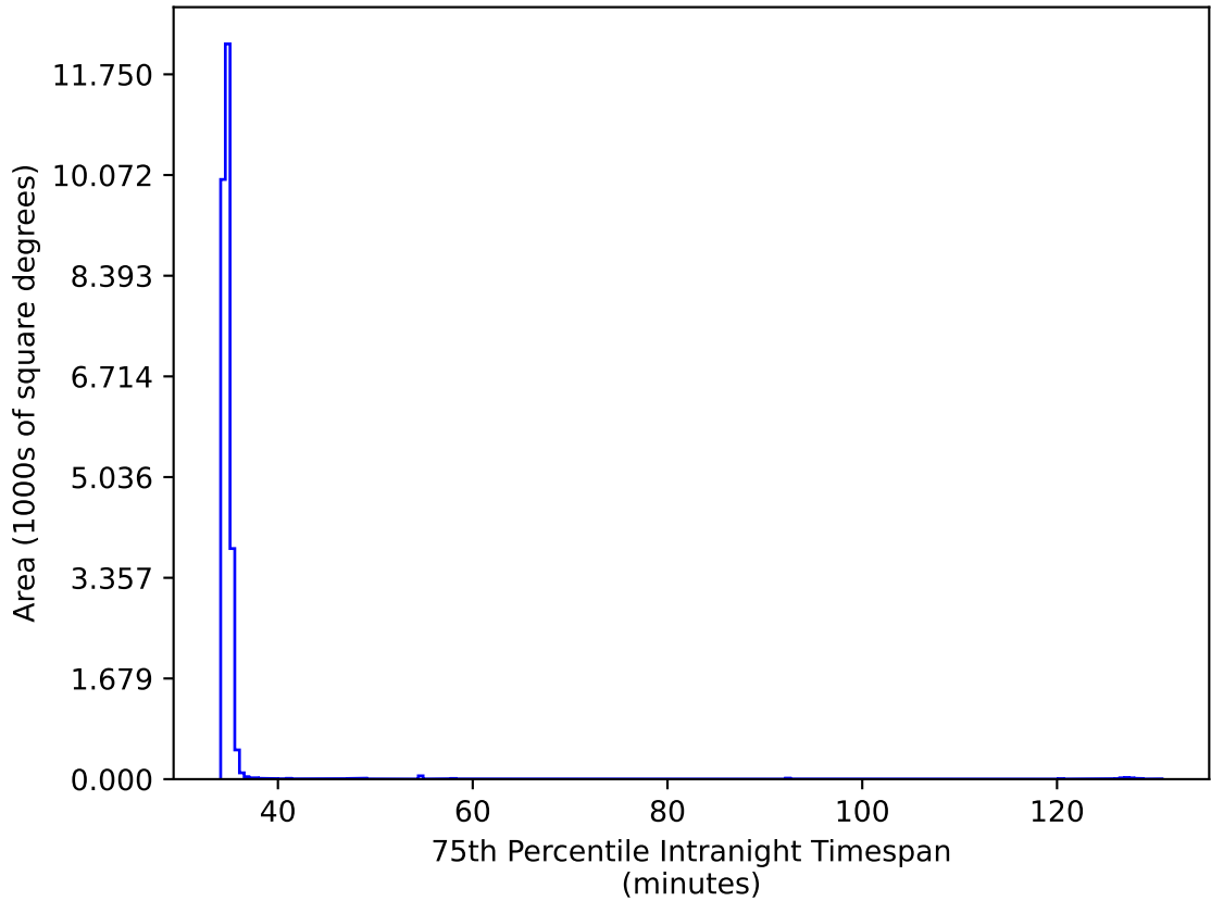
ddf_acor_sf10_lsf40_lsr10_v3.4_10yrs All sky iz bands: 75th Percentile Intranight Timespan
