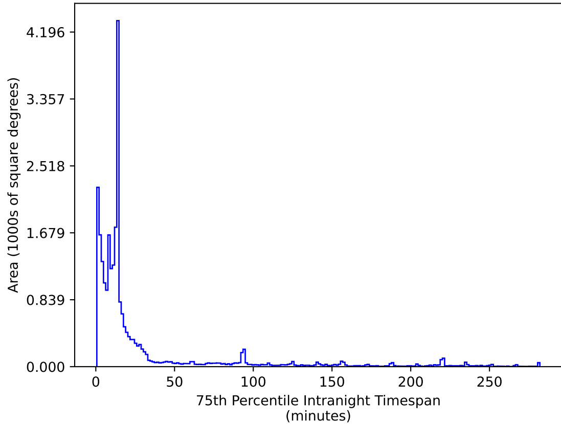
ddf_acor_sf10_lsf40_lsr10_v3.4_10yrs All sky i band: 75th Percentile Intranight Timespan
