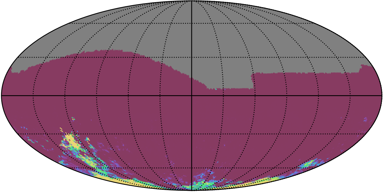
ddf_acor_sf10_lsf40_lsr10_v3.4_10yrs All sky gr bands: 75th Percentile Intranight Timespan
