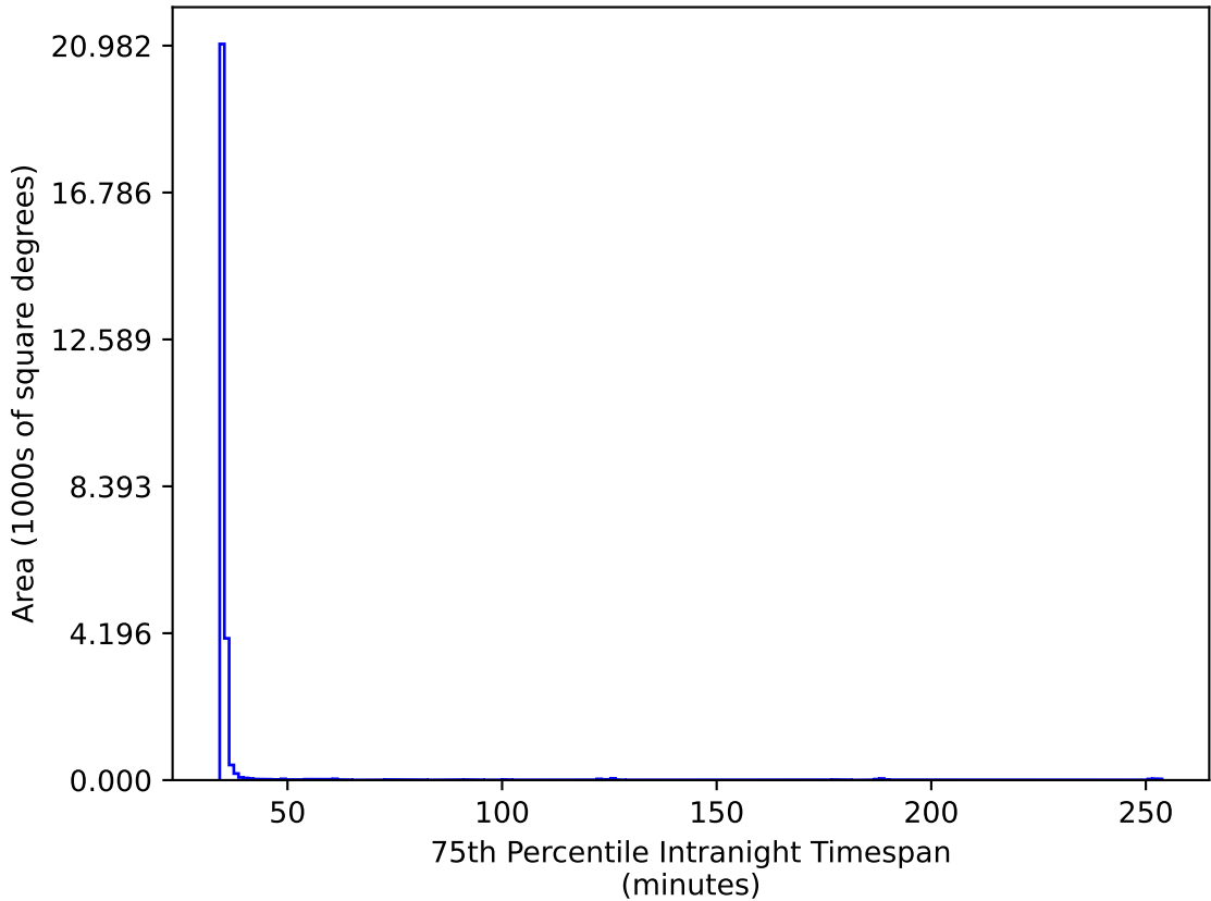
ddf_acor_sf10_lsf40_lsr10_v3.4_10yrs All sky gr bands: 75th Percentile Intranight Timespan
