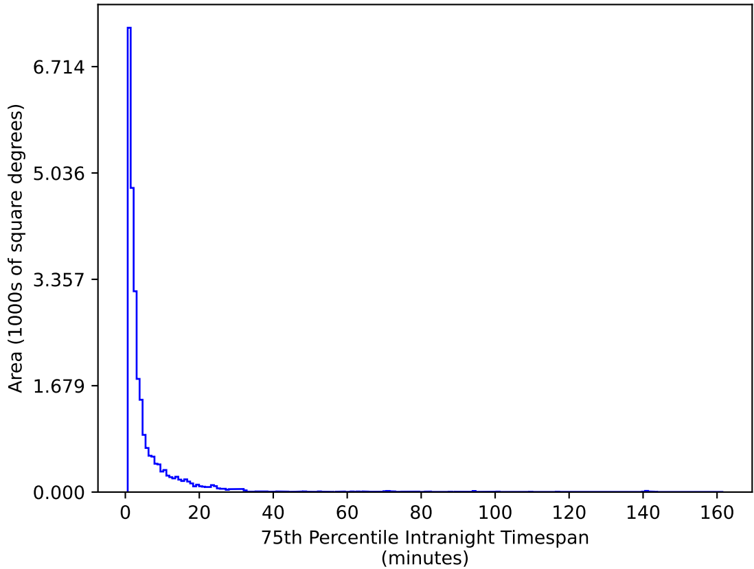
ddf_acor_sf10_lsf40_lsr10_v3.4_10yrs All sky g band: 75th Percentile Intranight Timespan
