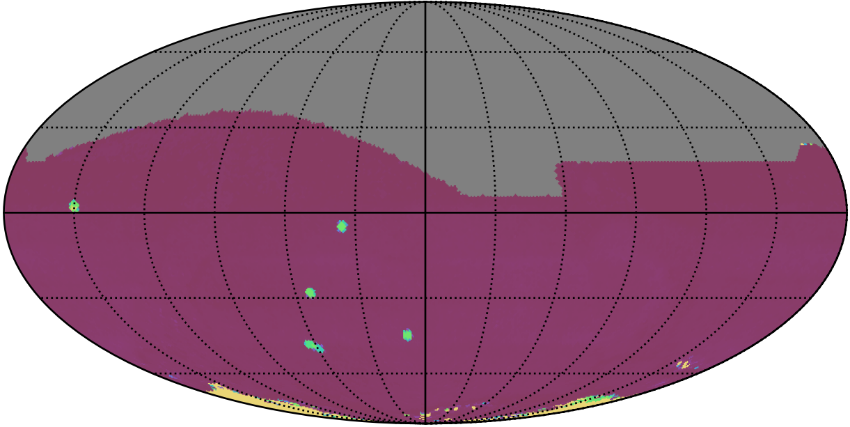
ddf_acor_sf10_lsf40_lsr10_v3.4_10yrs All sky all bands: 75th Percentile Intranight Timespan
