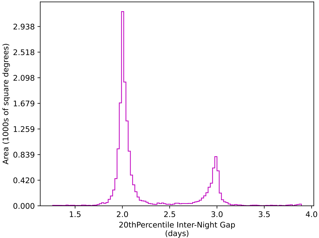
ddf_acor_sf10_lsf40_lsr10_v3.4_10yrs WFD z band: 20thPercentile Inter-Night Gap
