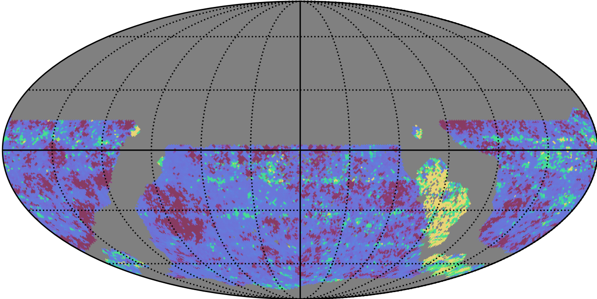
ddf_acor_sf10_lsf40_lsr10_v3.4_10yrs WFD y band: 20thPercentile Inter-Night Gap
