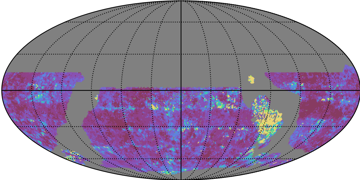
ddf_acor_sf10_lsf40_lsr10_v3.4_10yrs WFD u band: 20thPercentile Inter-Night Gap
