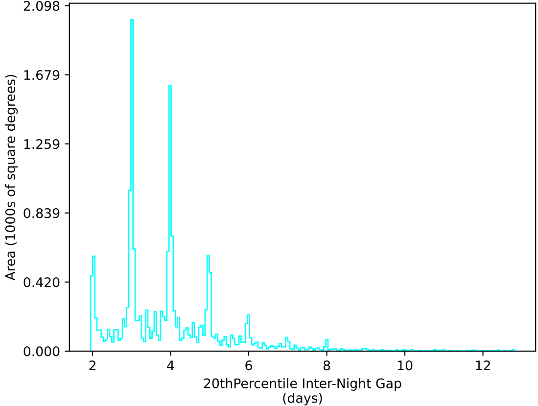
ddf_acor_sf10_lsf40_lsr10_v3.4_10yrs WFD u band: 20thPercentile Inter-Night Gap
