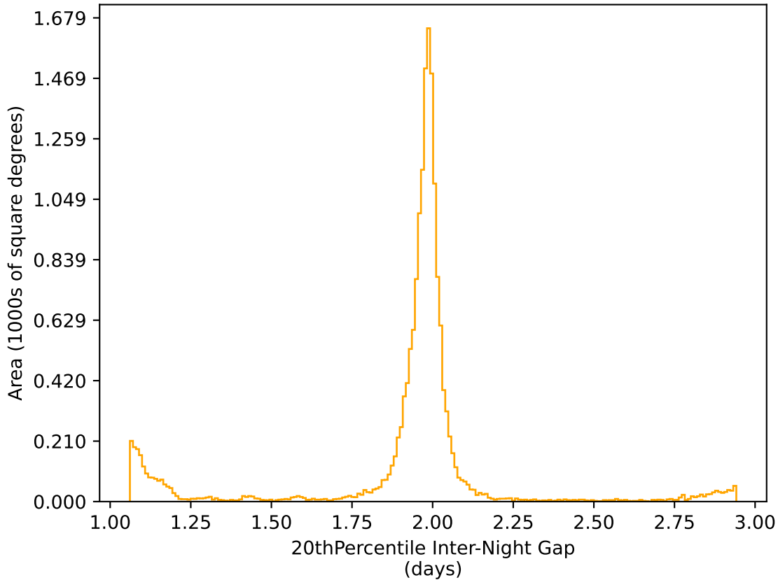
ddf_acor_sf10_lsf40_lsr10_v3.4_10yrs WFD r band: 20thPercentile Inter-Night Gap
