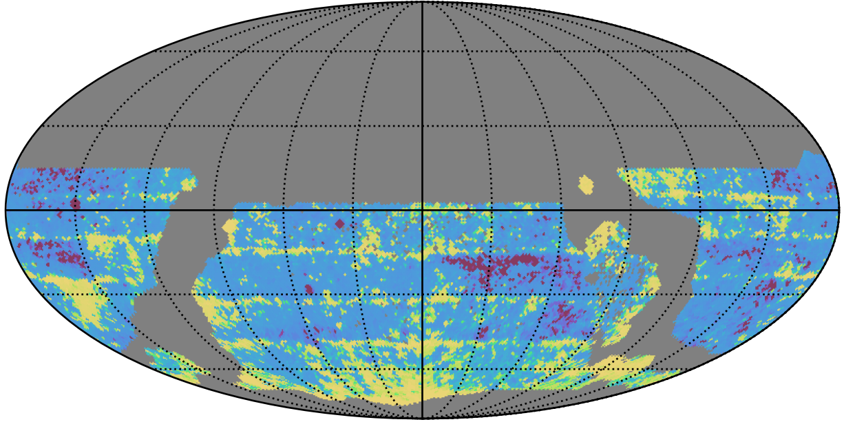
ddf_acor_sf10_lsf40_lsr10_v3.4_10yrs WFD i band: 20thPercentile Inter-Night Gap
