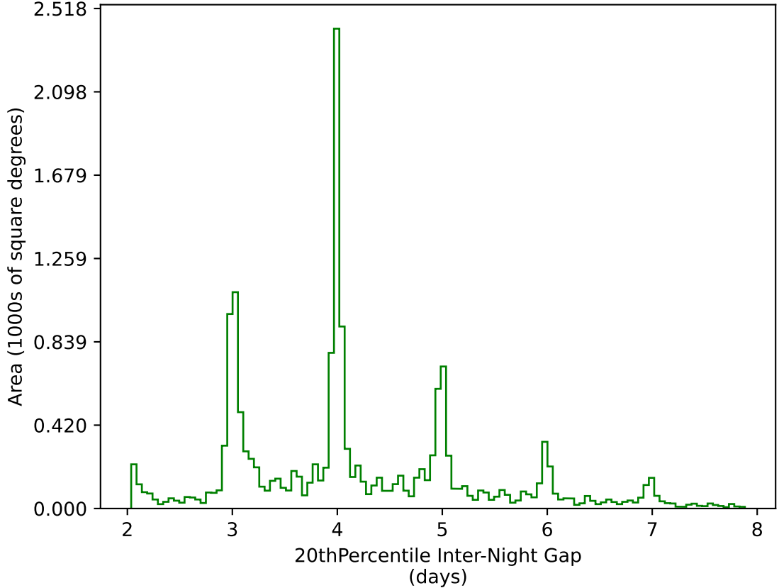
ddf_acor_sf10_lsf40_lsr10_v3.4_10yrs WFD g band: 20thPercentile Inter-Night Gap
