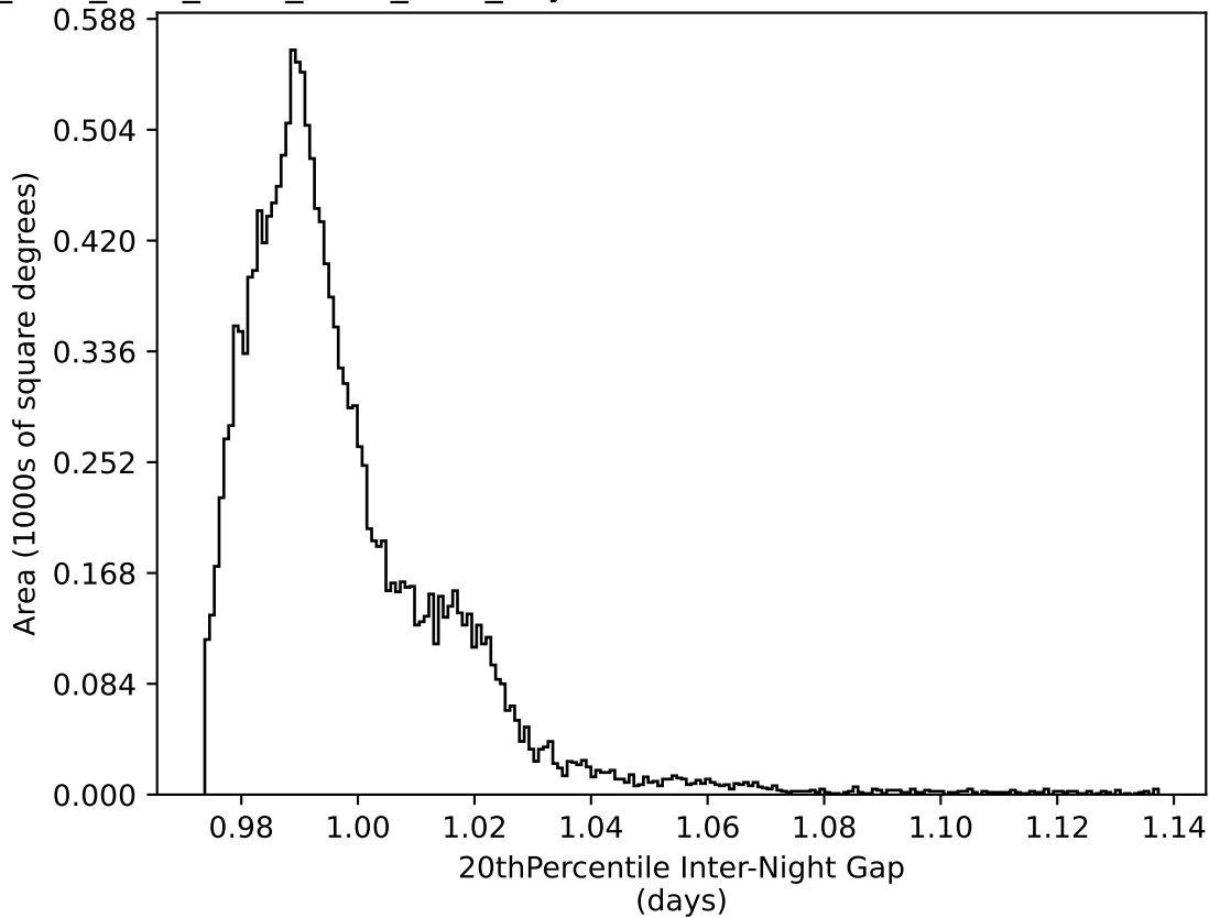
ddf_acor_sf10_lsf40_lsr10_v3.4_10yrs WFD all bands: 20thPercentile Inter-Night Gap
