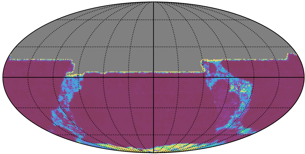
ddf_acor_sf10_lsf40_lsr10_v3.4_10yrs All sky y band: 20thPercentile Inter-Night Gap
