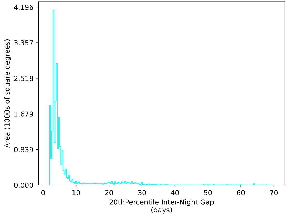
ddf_acor_sf10_ls40_lsr10_v3.4_10yrs All sky u band: 20thPercentile Inter-Night Gap
