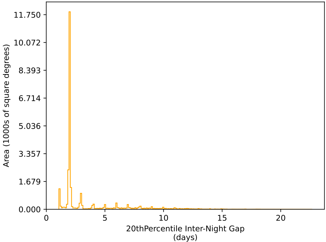
ddf_acor_sf10_ls40_lsr10_v3.4_10yrs All sky r band: 20thPercentile Inter-Night Gap
