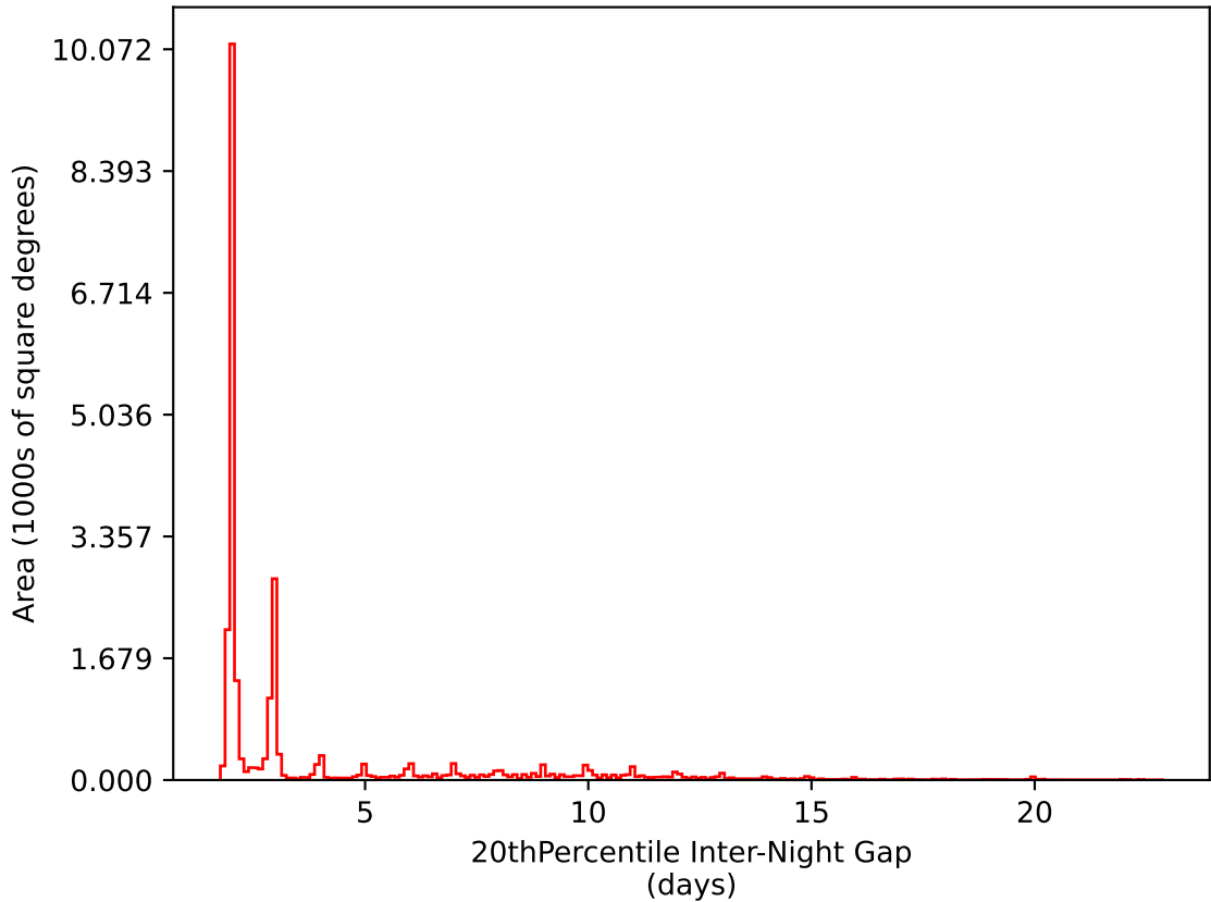
ddf_acor_sf10_lsf40_lsr10_v3.4_10yrs All sky i band: 20thPercentile Inter-Night Gap
