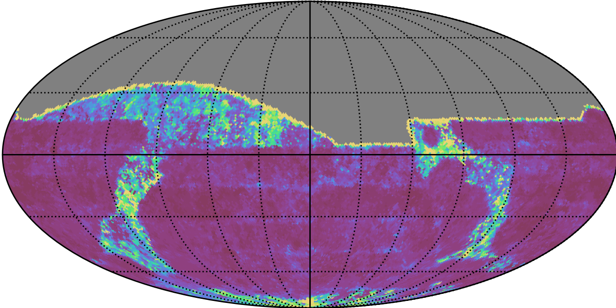
ddf_acor_sf10_lsf40_lsr10_v3.4_10yrs All sky g band: 20thPercentile Inter-Night Gap
