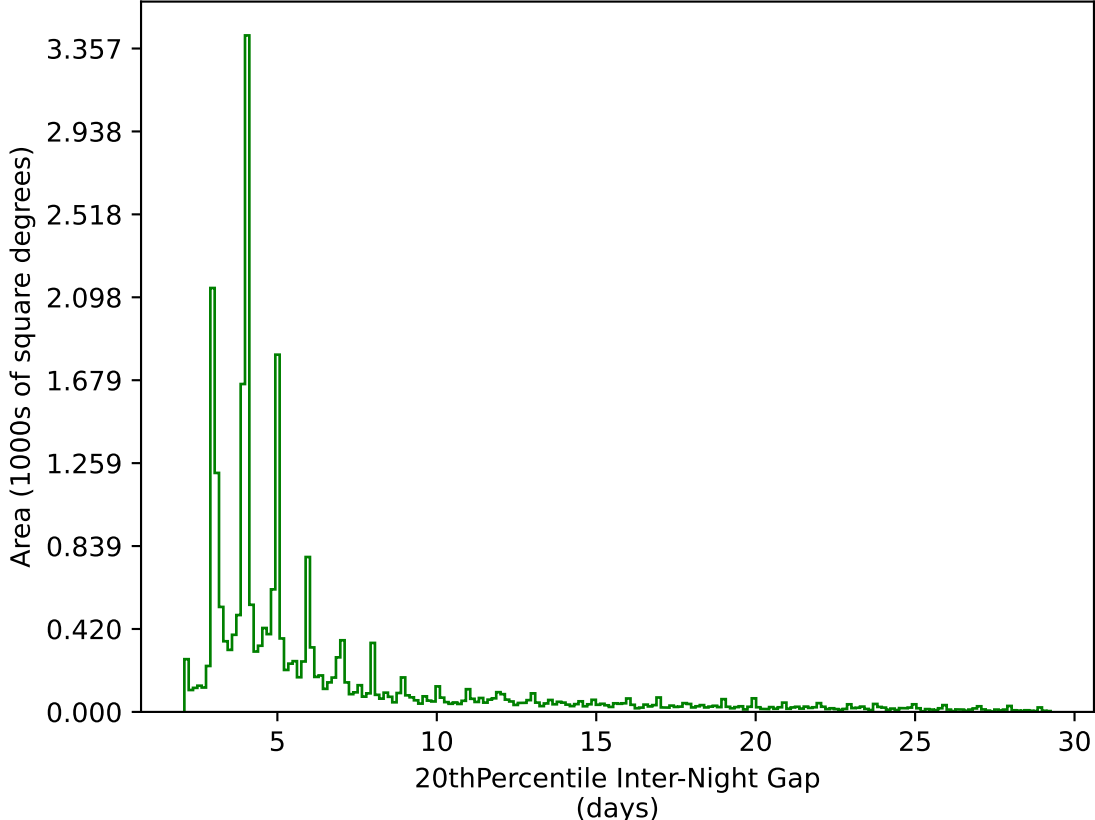
ddf_acor_sf10_lsf40_lsr10_v3.4_10yrs All sky g band: 20thPercentile Inter-Night Gap
