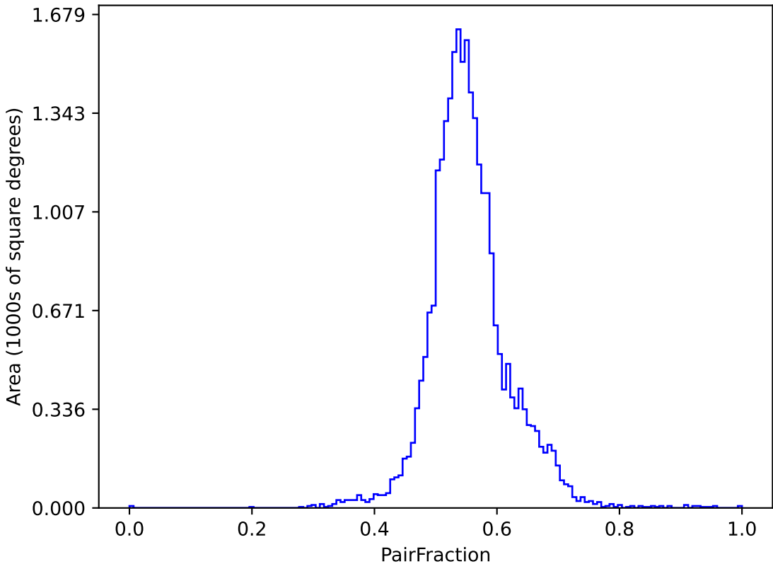
ddf_acor_sf10_lsf40_lsr10_v3.4_10yrs (g or r or i): PairFraction
