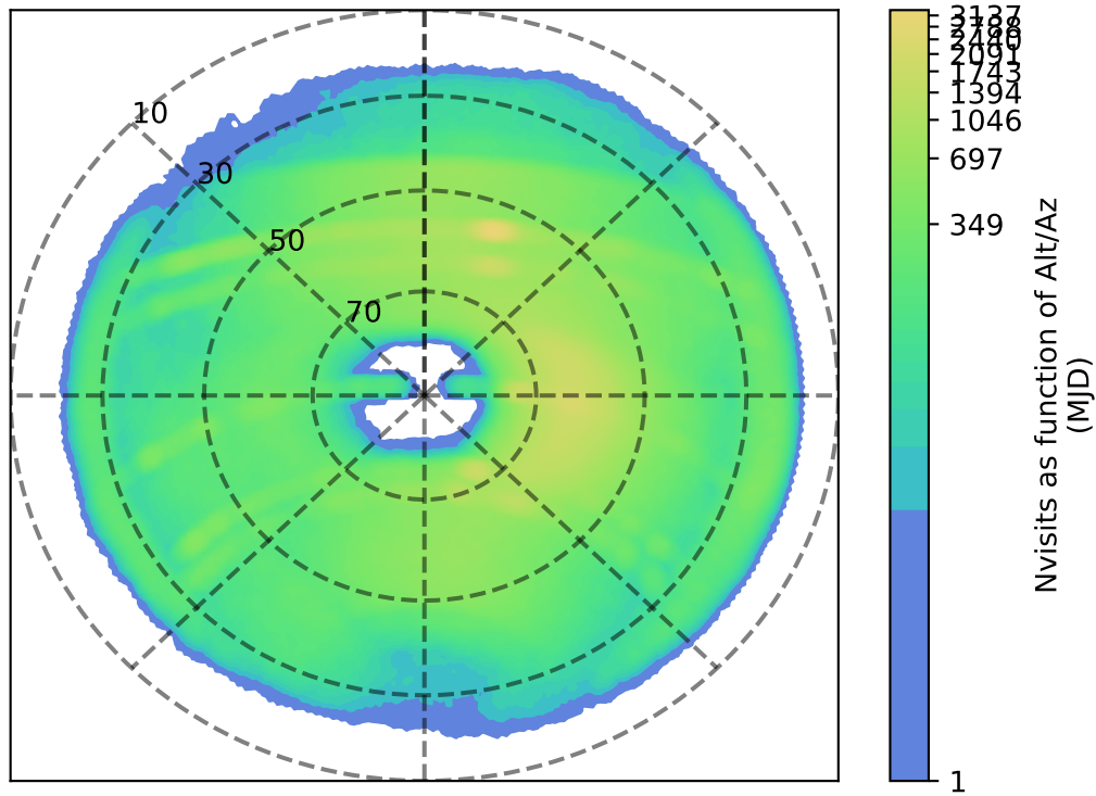
ddf_acor_sf10_ls40_lsr10_v3.4_10yrs z: Nvisits as function of Alt/Az
