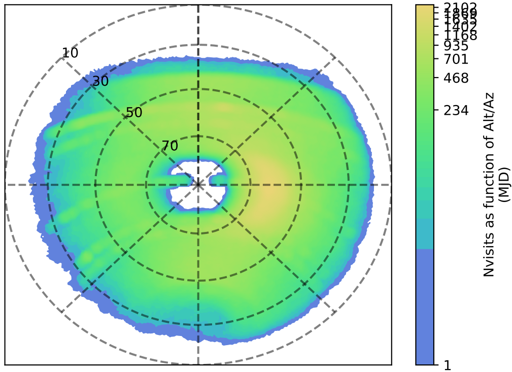
ddf_acor_sf10_lsf40_lsr10_v3.4_10yrs y: Nvisits as function of Alt/Az
