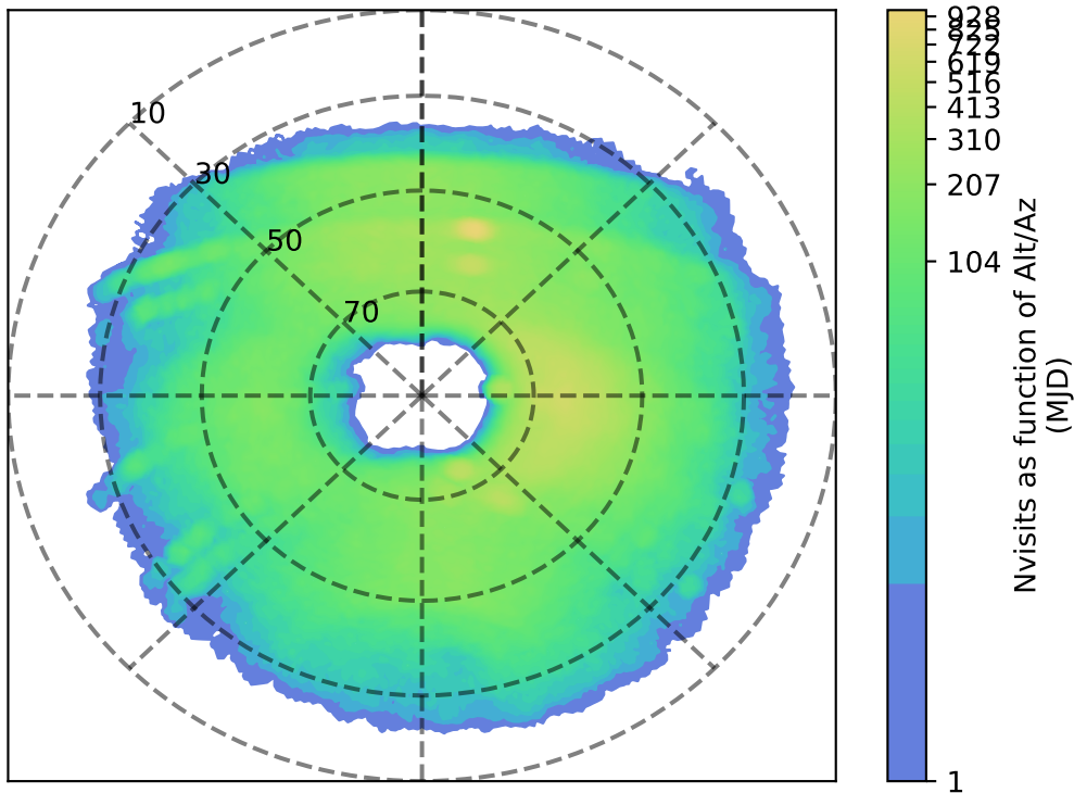
ddf_acor_sf10_ls40_isr10_v3.4_10yrs u: Nvisits as function of Alt/Az
