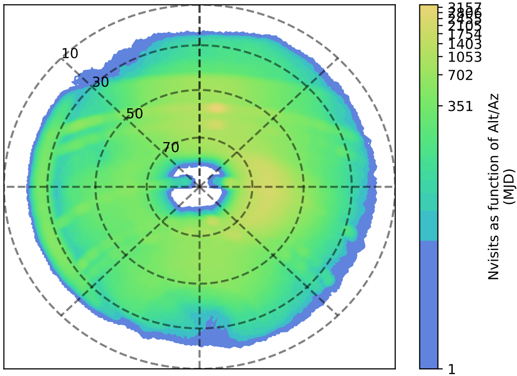
ddf_acor_sf10_ls40_lsr10_v3.4_10yrs r: Nvisits as function of Alt/Az
