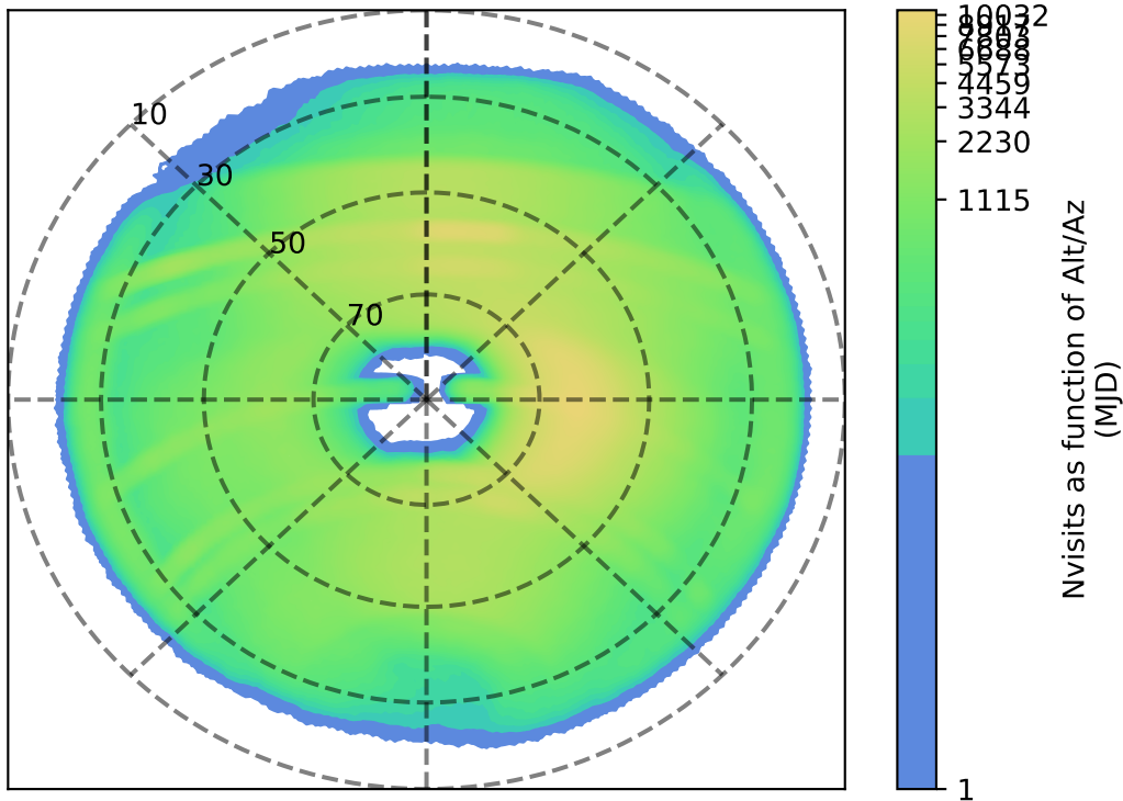
ddf_acor_sf10_lsf40_lsr10_v3.4_10yrs : Nvisits as function of Alt/Az
