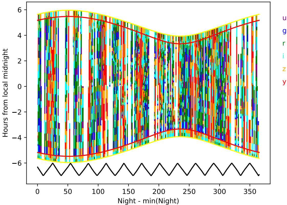
ddf_acor_sf10_lsf40_lsr10_v3.4_10yrs year 7-8: Hourglass
