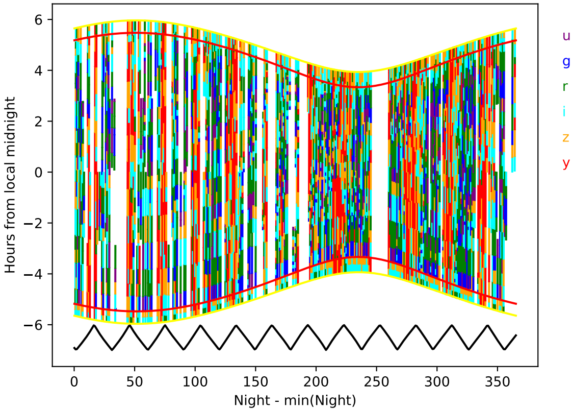
ddf_acor_sf10_lsf40_lsr10_v3.4_10yrs year 5-6: Hourglass
