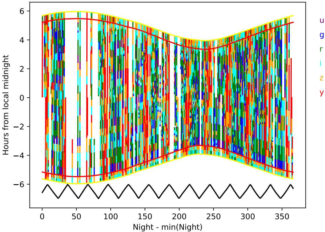
ddf_acor_sf10_lsf40_lsr10_v3.4_10yrs year 3-4: Hourglass
