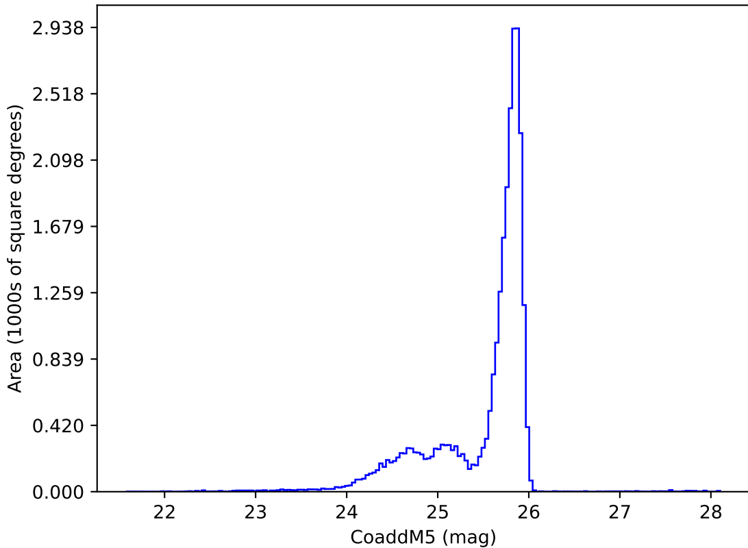
ddf_acor_sf10_lsf40_lsr10_v3.4_10yrs z: CoaddM5
