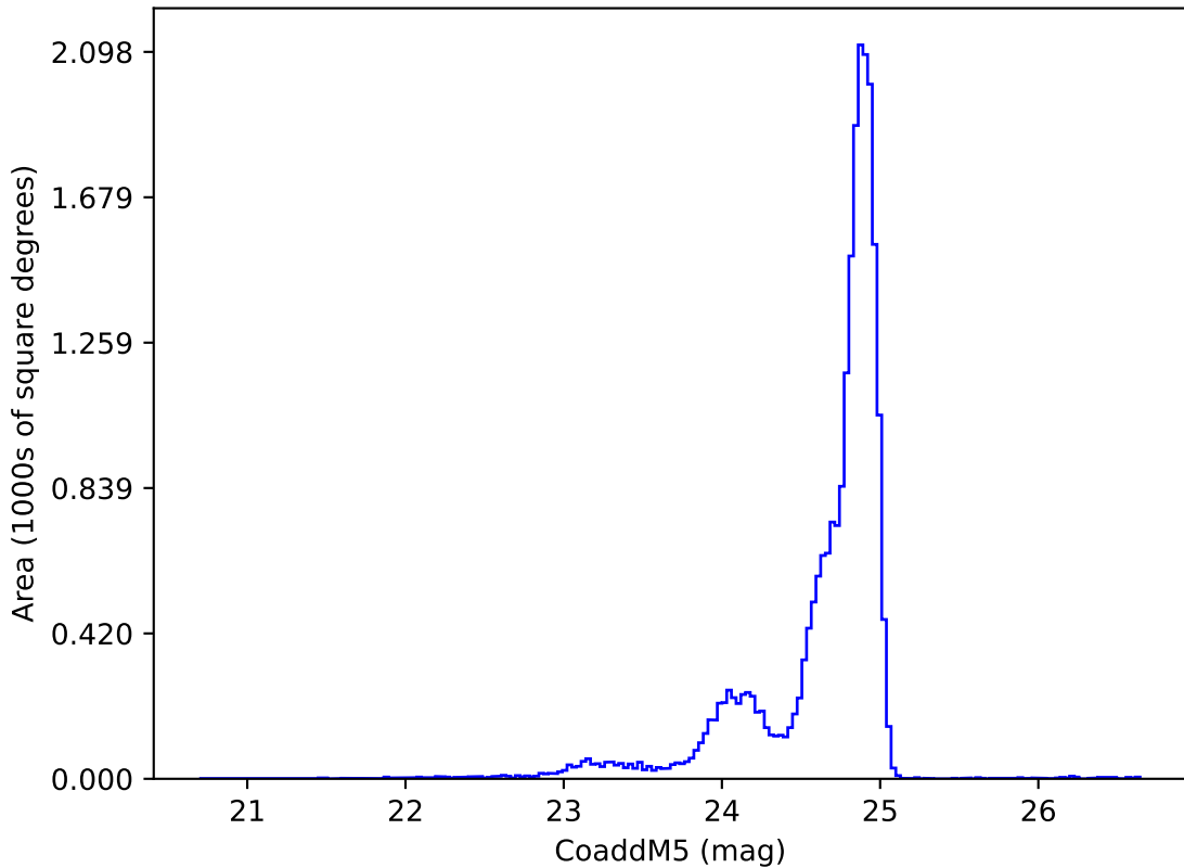
ddf_acor_sf10_lsf40_lsr10_v3.4_10yrs y: CoaddM5
