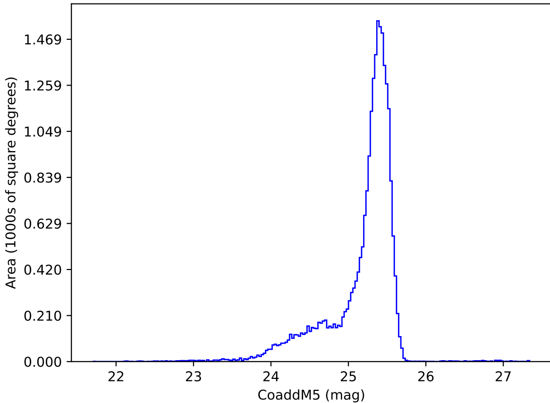
ddf_acor_sf10_lsf40_lsr10_v3.4_10yrs u: CoaddM5
